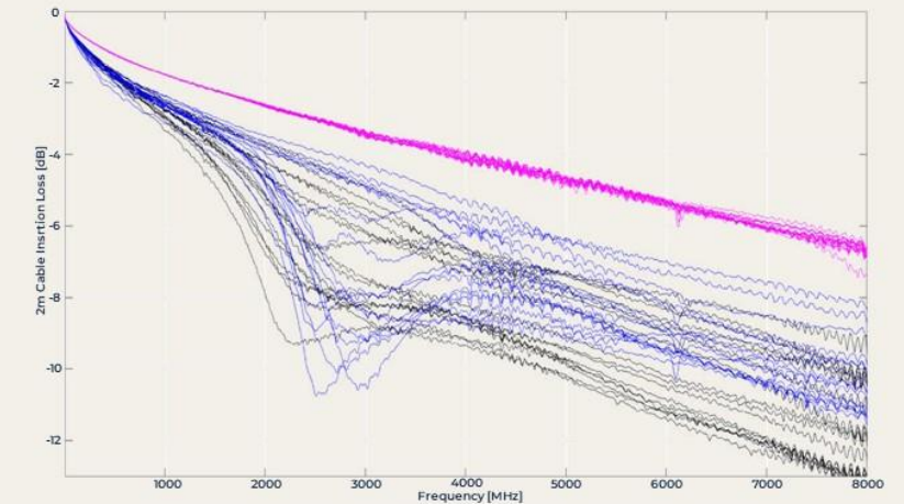
Dynamic Coax Insertion Loss (IL) Degradation: Aging leads to major Insertion Loss degradation and distortions
